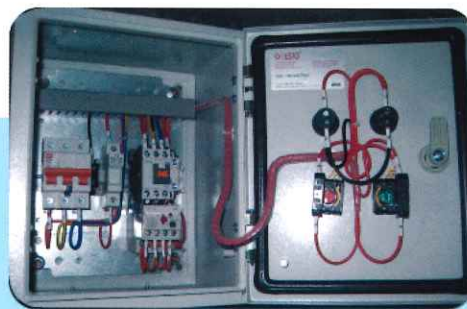
D.O.L Control Panel
